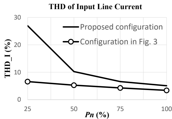
Figure 10. Comparison of the THD in the input line current between the proposed configuration and the configuration shown in Figure 3.
