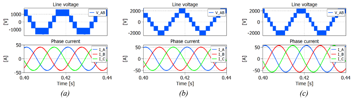
Figure 6. Output line voltage and phase current of 4L-NPC inverter. (a): 50% load; (b): 75% load; (c): full load.
