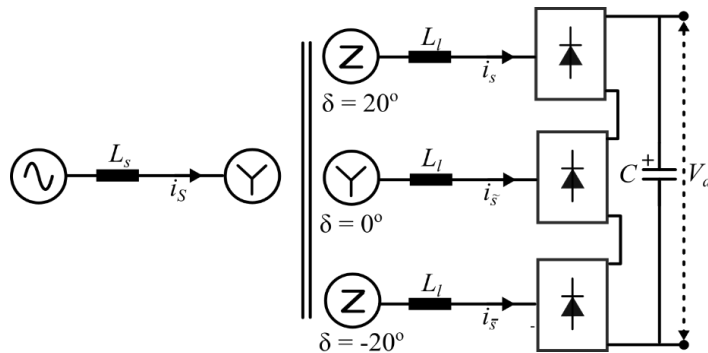
Figure 3. Block diagram of an 18-pulse diode rectifier.
