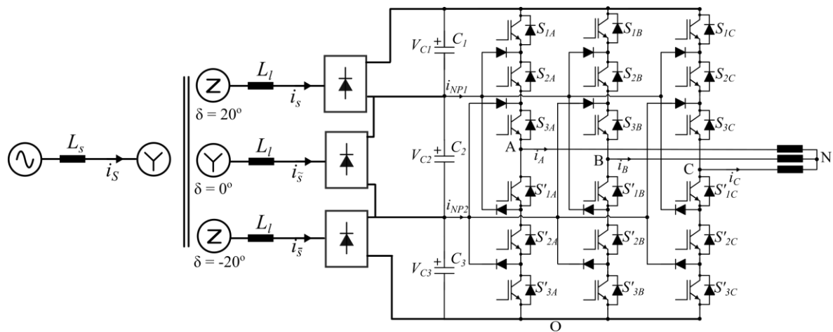
Figure 4. The proposed diagram of the 18-Pulse Diode Rectifier Fed 4L-NPC Inverter.
